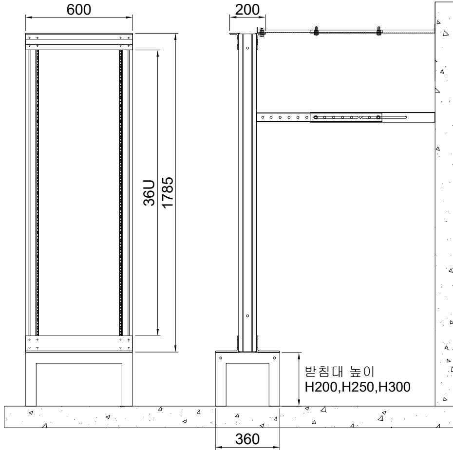
FRONT VIEW
