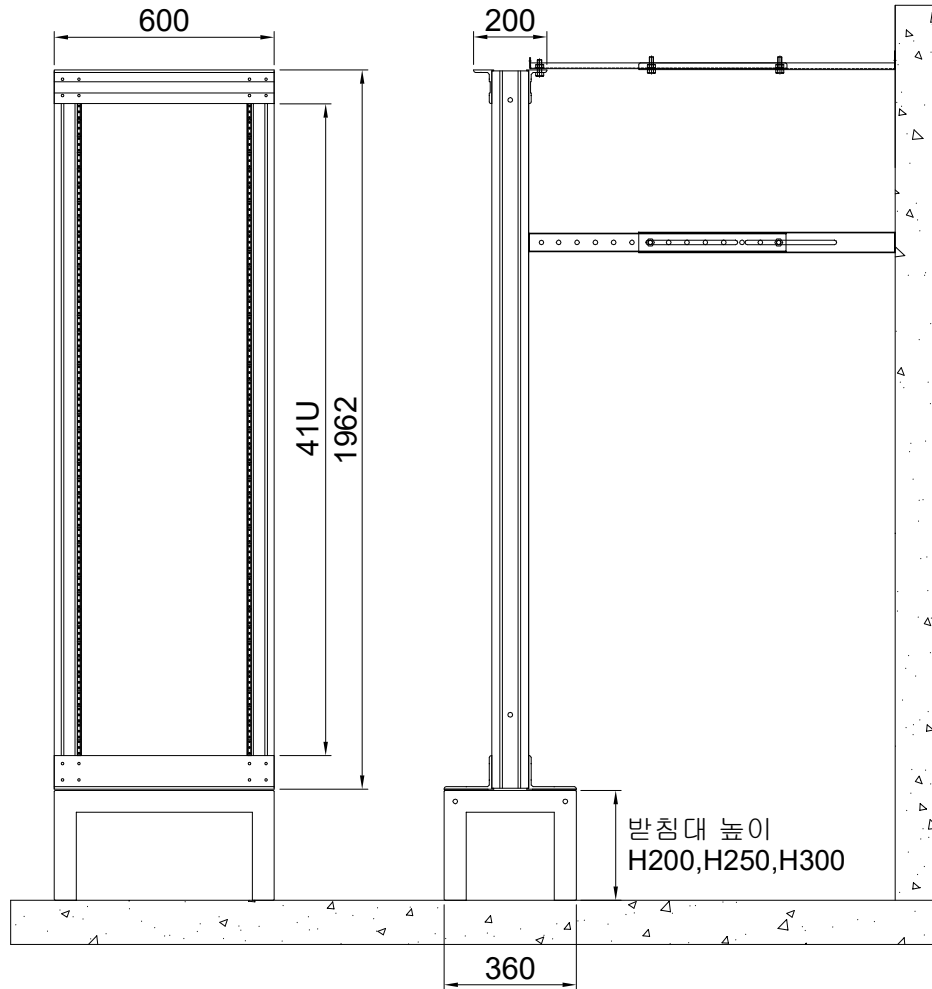
FRONT VIEW
