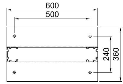
BASE VIEW
