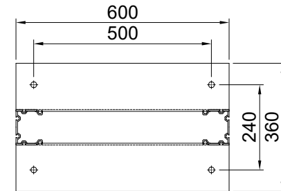
BASE VIEW
