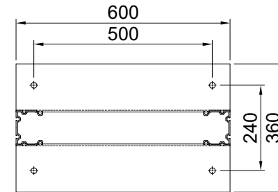
BASE VIEW
