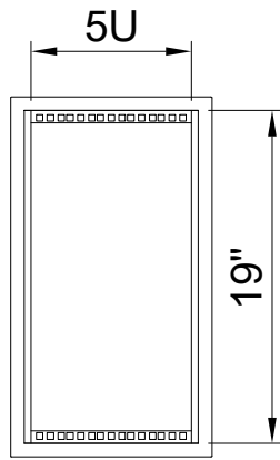
FRONT VIEW (Door Removed)
